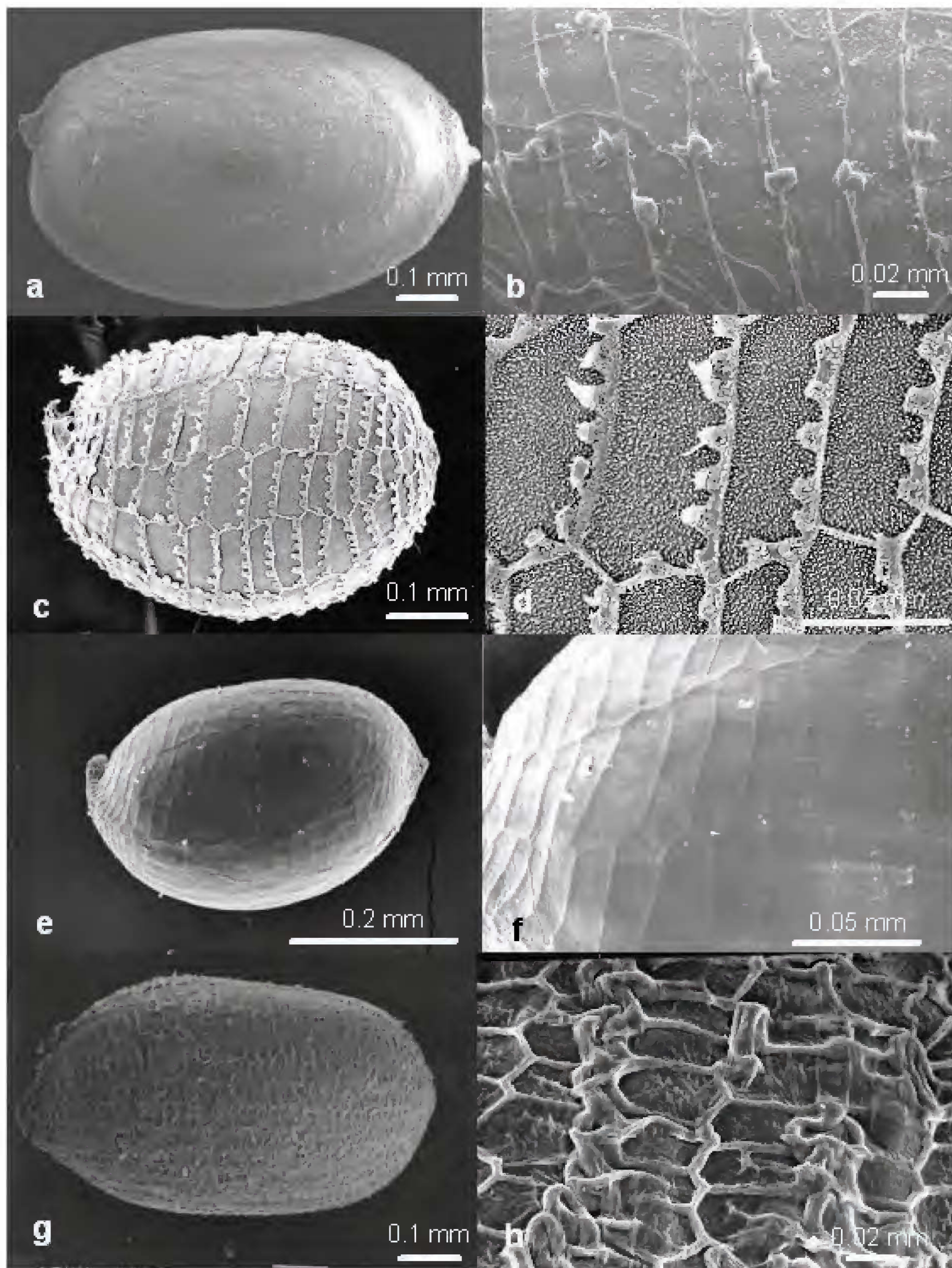
Fig. 2. Seed and seed surface: Eriocaulon aloefolium a, b ; E. athertonense c, d ; E. australasicum e, f ; E. australe g, h . Material used: a-b from Davies 418 ; c-d from Blake 18800 ; e-f from Mueller K001056248 ; g-h from Durrington 1441 .
